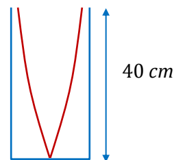
pipe in fundamental mode
